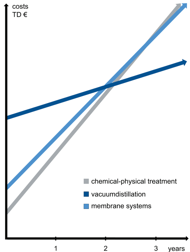
Fig. 4: Comparison of life cycle costs of process water treatment systems
