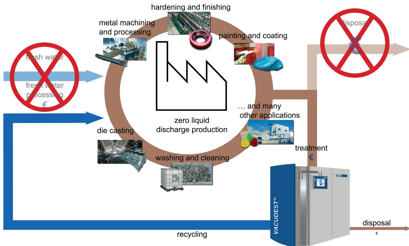
Fig. 1: Vacuum distillation saves money
