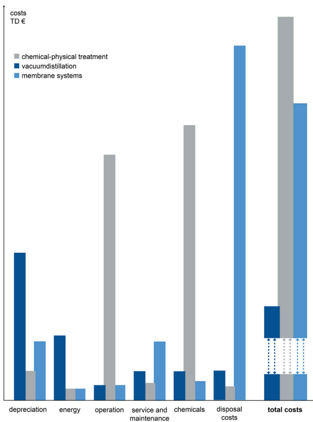
Fig. 3: Comparison of operation costs for process water treatment systems
